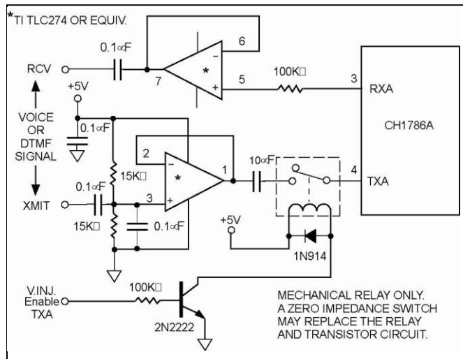
Figure 4. Voice/Tone Injection.
