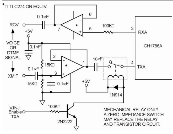
Figure 4. Voice/Tone Injection.
