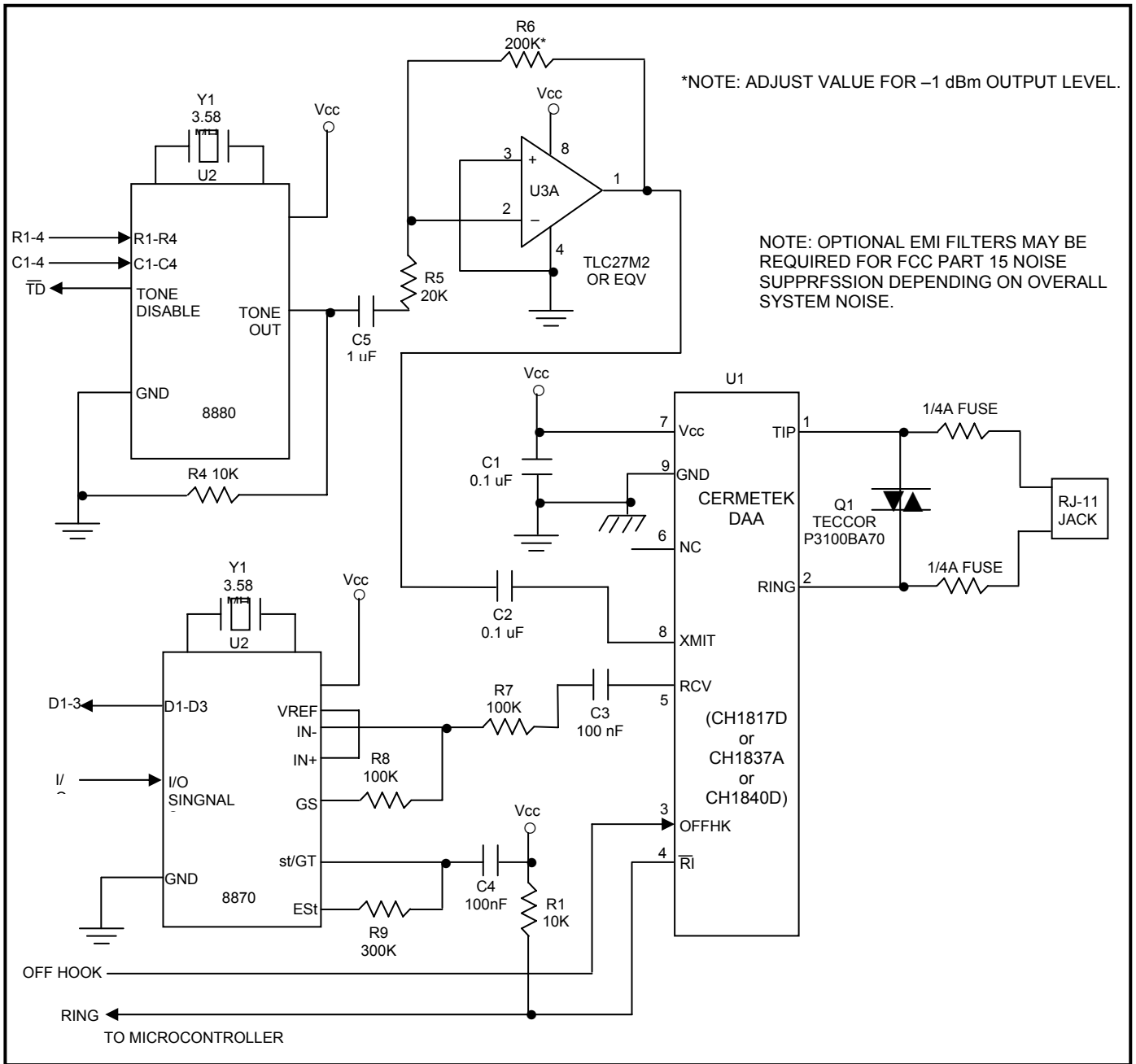
Figure 2. Implementation Using Separate DTMF Transmitter and Receiver Circuits.
